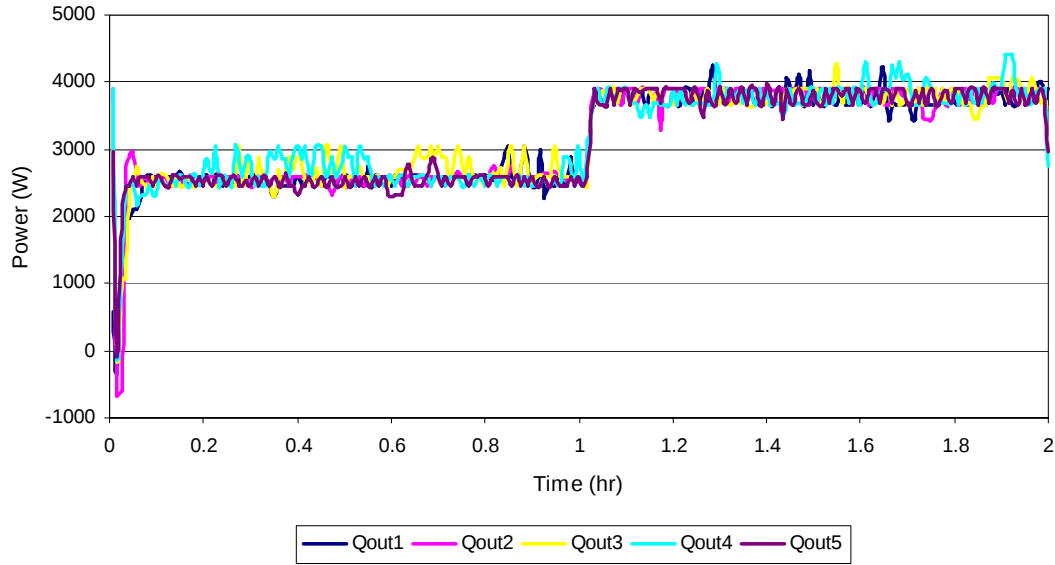
Figure 5. Output from the five repeatability test trials overlaid.
